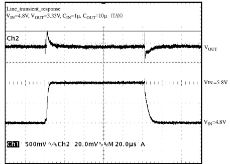
Figure 14. Line Transient Response
