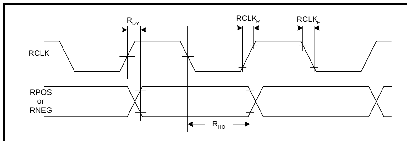
FIGURE 8. RECEIVE CLOCK AND OUTPUT DATA TIMING
