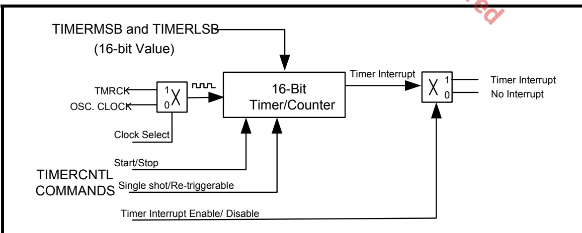
FIGURE 14. TIMER/COUNTER CIRCUIT
