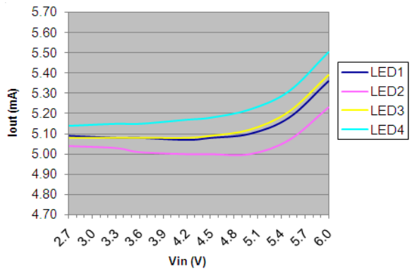
Fig. 15: Line Regulation @ T_A = -40^\circ\text{C} DAC = 001010 (5mA)
