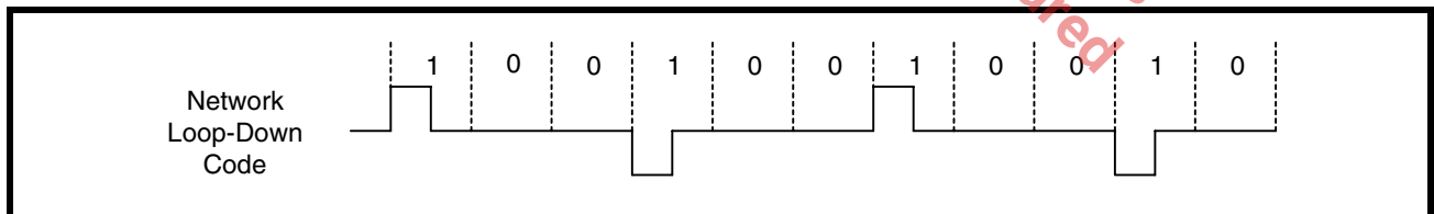
FIGURE 35. NETWORK LOOP DOWN CODE GENERATION
