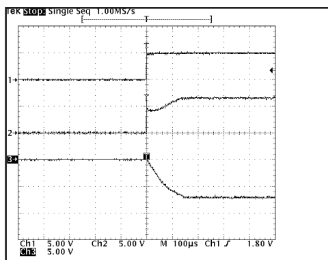
Figure 6, Charge pump outputs at start up (Ch1 = Vcc, Ch2 = V+, Ch3 = V-, Ch4 = V-).
