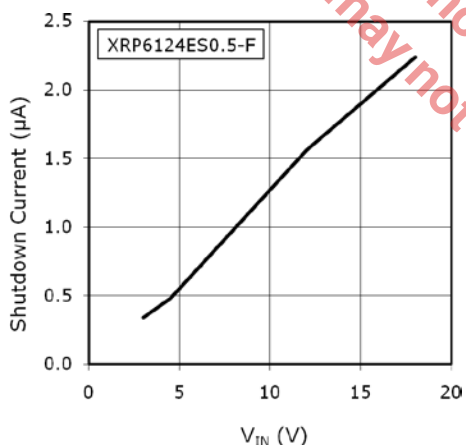
Fig. 18: Shutdown current versus V_{IN} , V_{EN} = 0V
