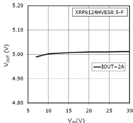
Fig. 11: Line Regulation
