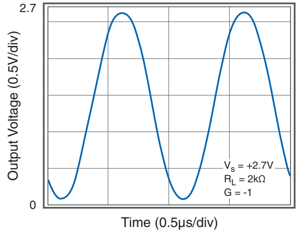
Output Swing
