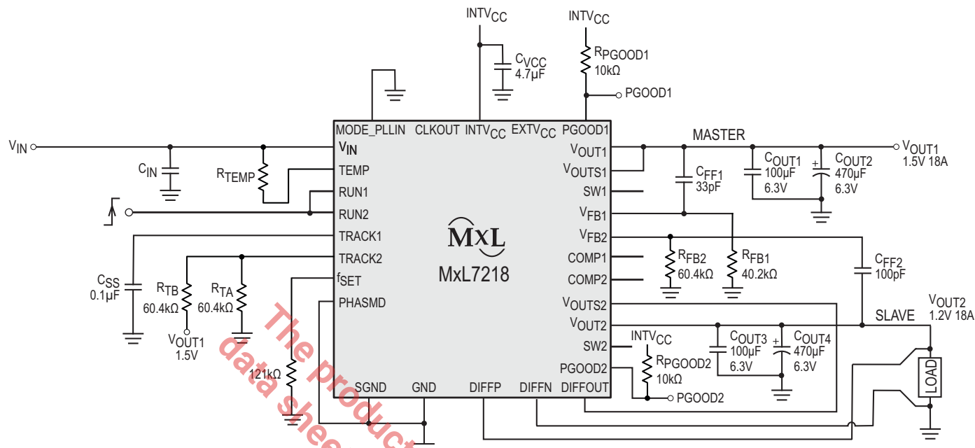
Figure 24: Example of Output Tracking Application Circuit
