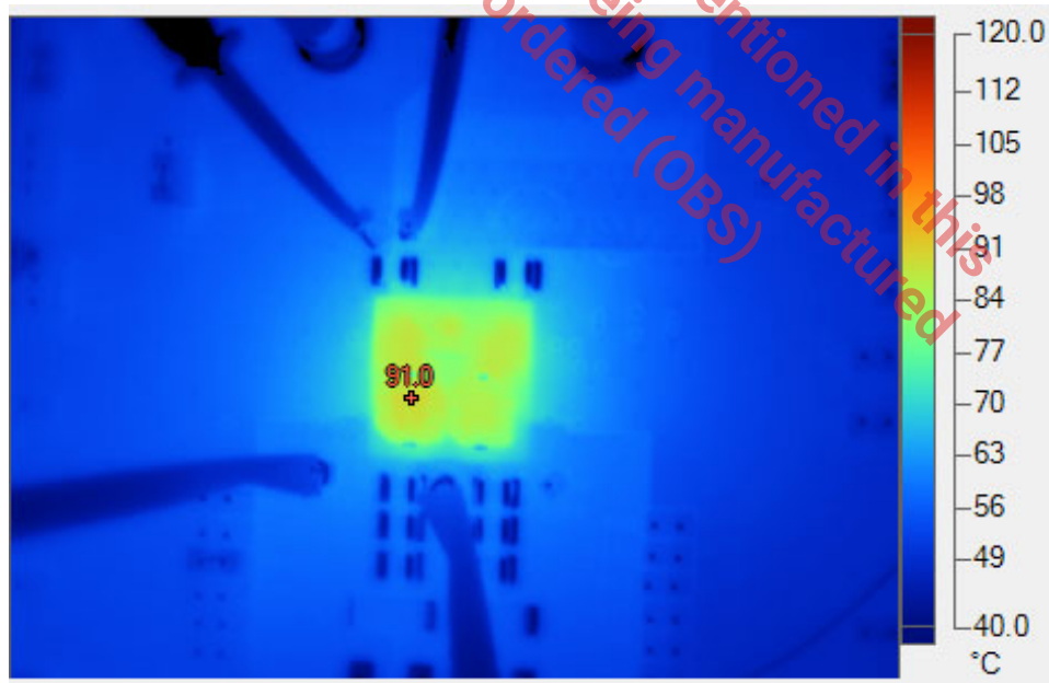
Figure 33: Thermal Image 12V to 1V, 50A with No Air Flow (1)
