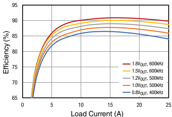
Figure 5: Efficiency: Single Phase, V_{IN} = 12V
