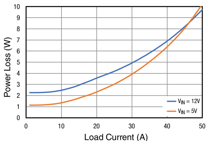
Figure 38: 1.5V Output Power Loss
