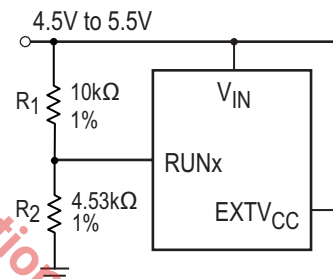
Figure 30: Self-Start for V_{IN} Range of 4.5V to 5.5V
