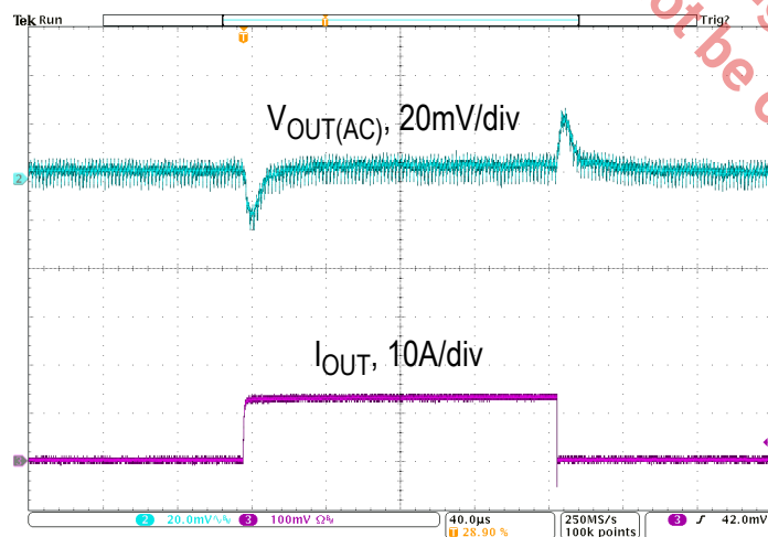
Figure 10: 12V to 1.5V, 600kHz, 12.5A Load Step, 10A/μs Step-Up and Step-Down
