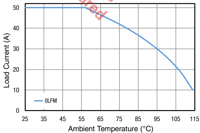
Figure 42: 5V to 0.9V Current Derating
