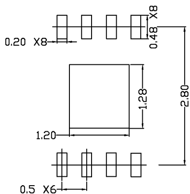
TYPICAL RECOMMENDED STENCIL
