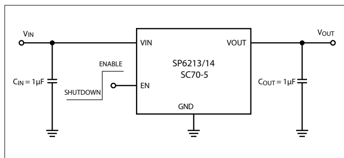
Figure 1: Typical Application
