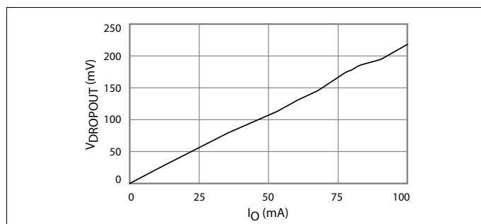
Figure 2: Dropout Voltage vs Output Current
