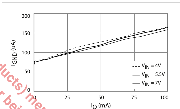
Figure 14: Ground Current vs Output Current
