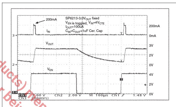
Figure 26: Inrush Current ( V_{IN} = 4V , I_{OUT} = 100\mu A )
