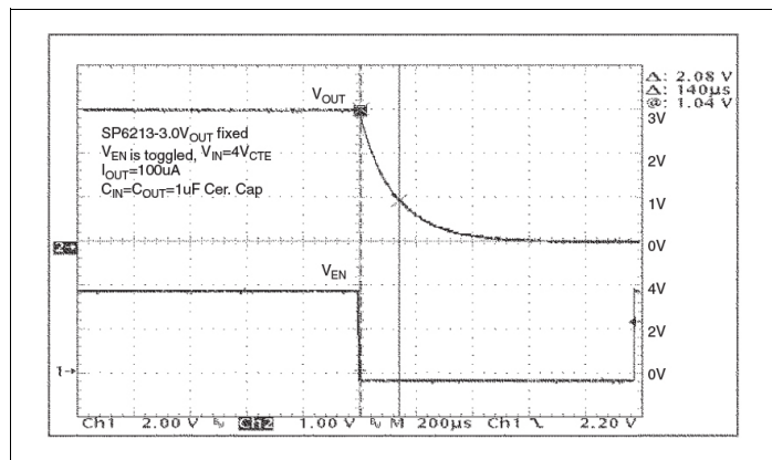
Figure 23: Turn-off Time ( V_{IN} = 4V , I_{OUT} = 100\mu A )
