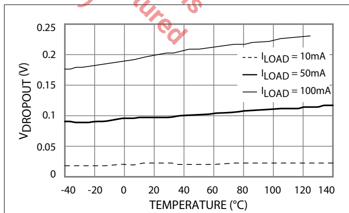
Figure 10: Dropout Voltage vs Temperature
