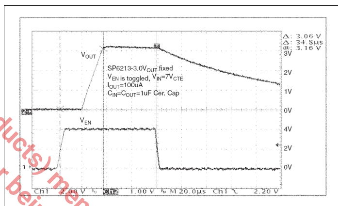
Figure 20: Turn-on Characteristic ( V_{IN} = 7V , I_{OUT} = 100\mu A )
