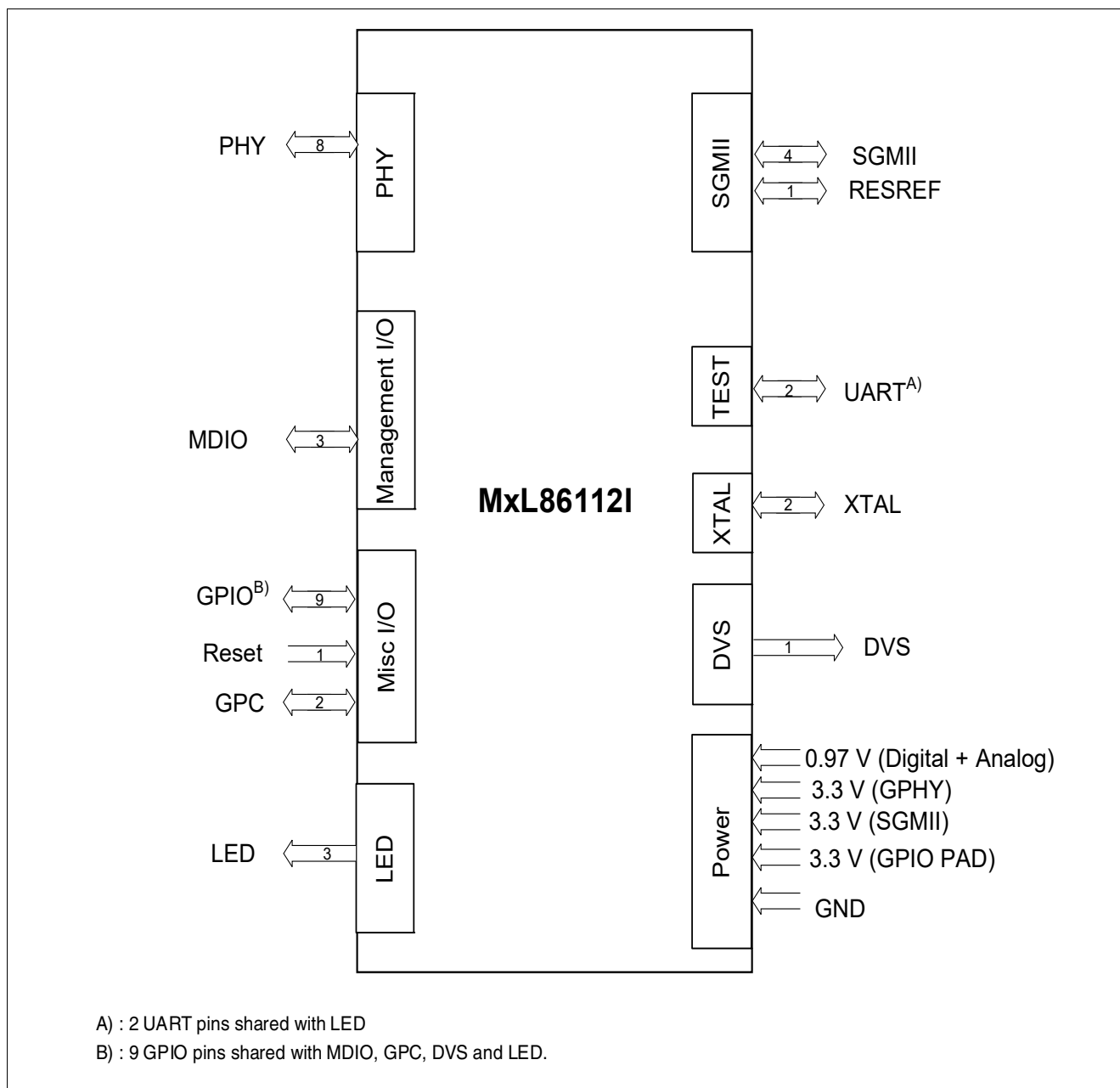
Figure 2 Ethernet PHY MxL86112I External Signals Overview
