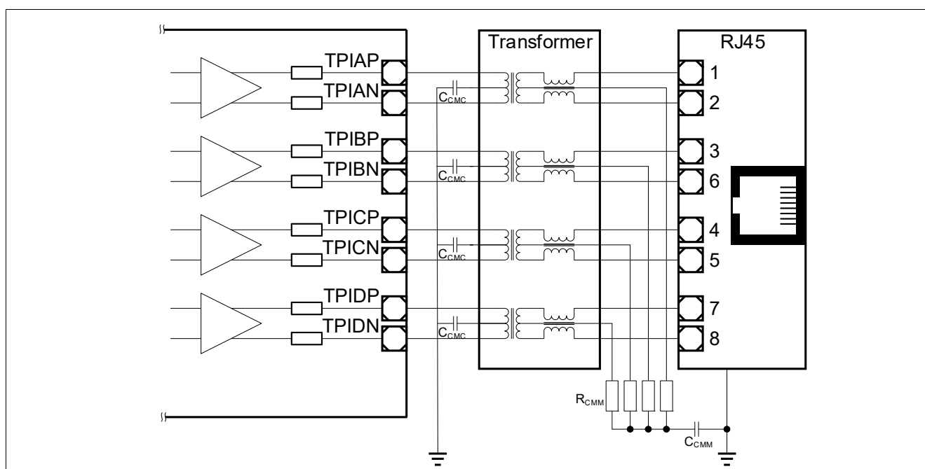
Figure 5 Twisted-Pair Interface of MxL86112I Including Transformer and RJ45 Plug
