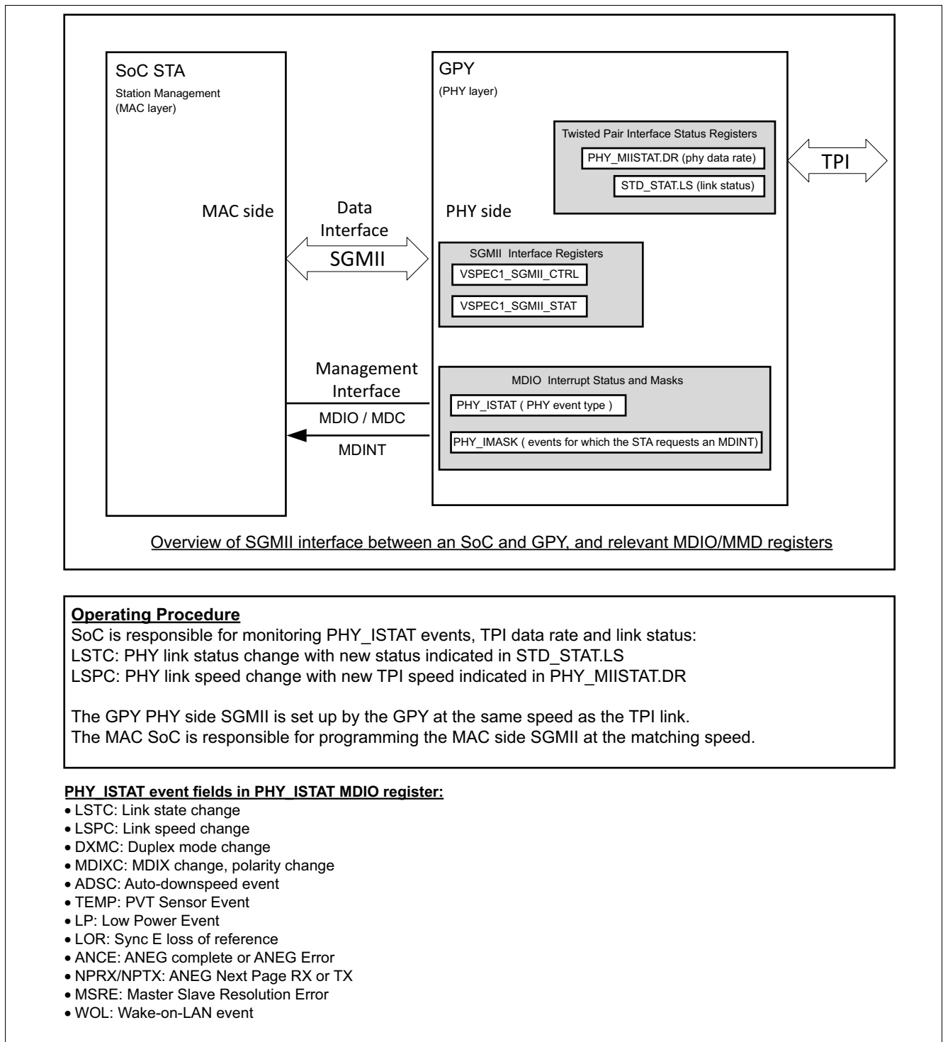
Figure 9 MxL86112I SGMII Configuration and Status Registers
