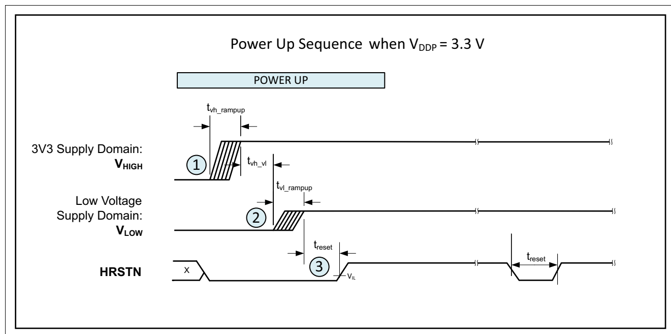
Figure 16 Timing Diagram for the Reset Sequence when V_{DDP} = 3.3 V
