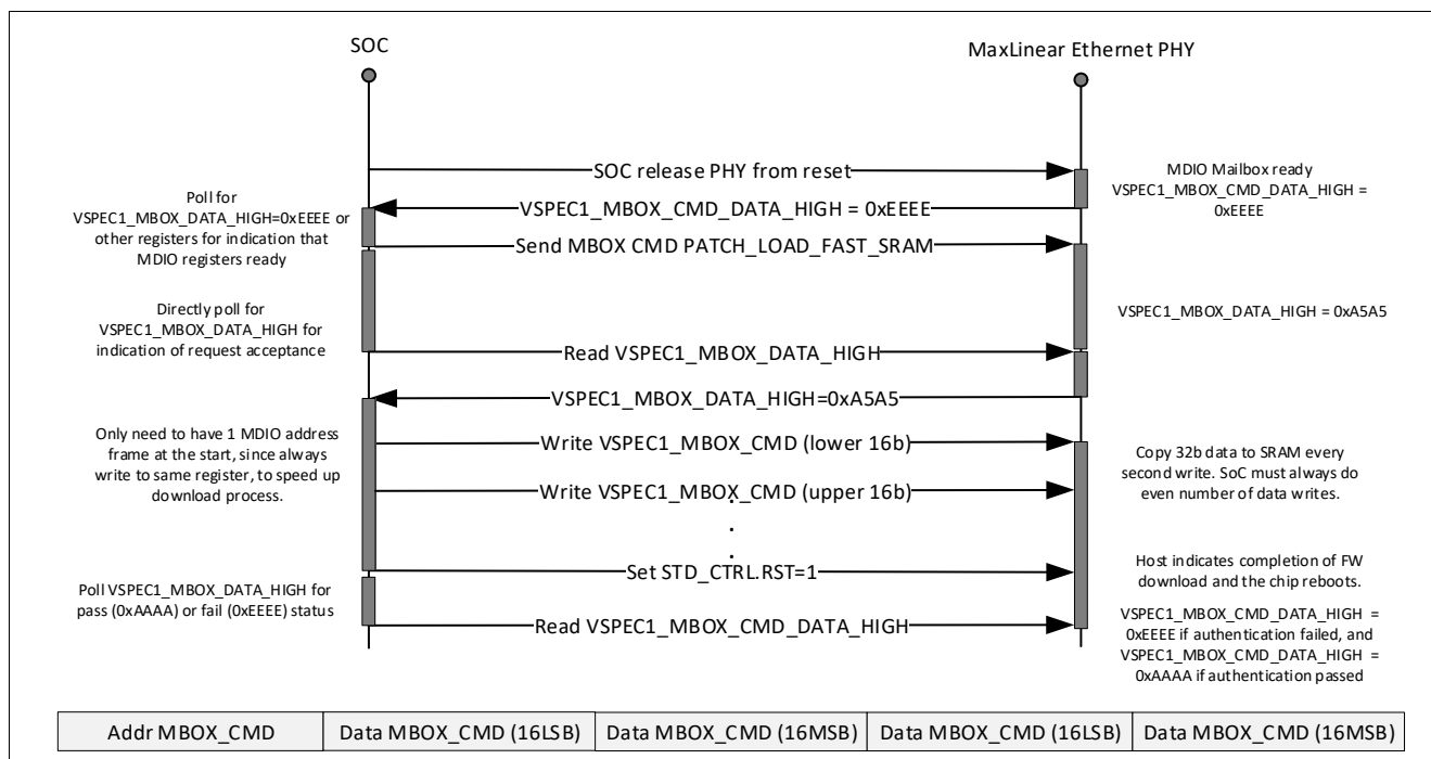
Figure 15 Firmware upgrade
