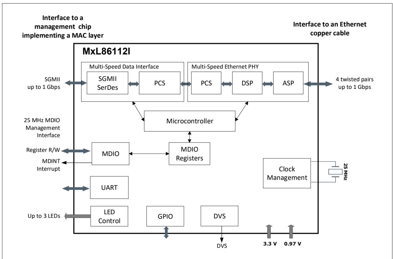
Figure 1 Ethernet PHY MxL86112I Block Diagram
