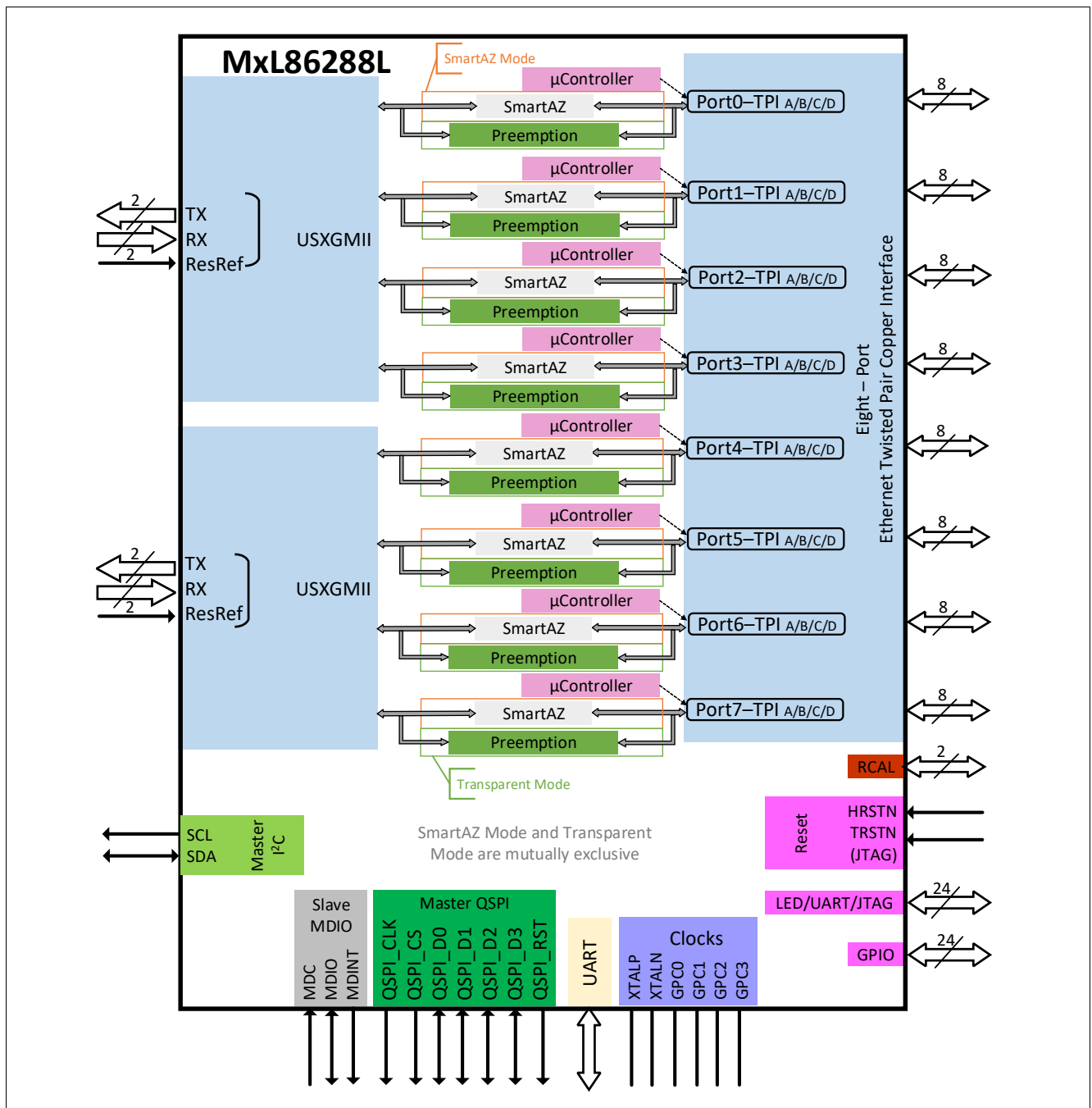
Figure 1 MxL86288L Block Diagram
