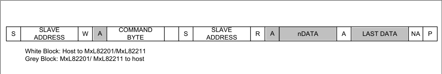
Figure 5: Master Reads From Slave
