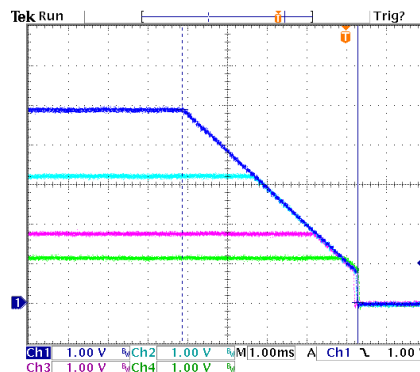
Fig. 11: Sequential Soft-Stop Configuration CH1:5V CH2:3.3V CH3:1.8V CH4:1.2V Vout Shutdown = 0.8V, 3A load
