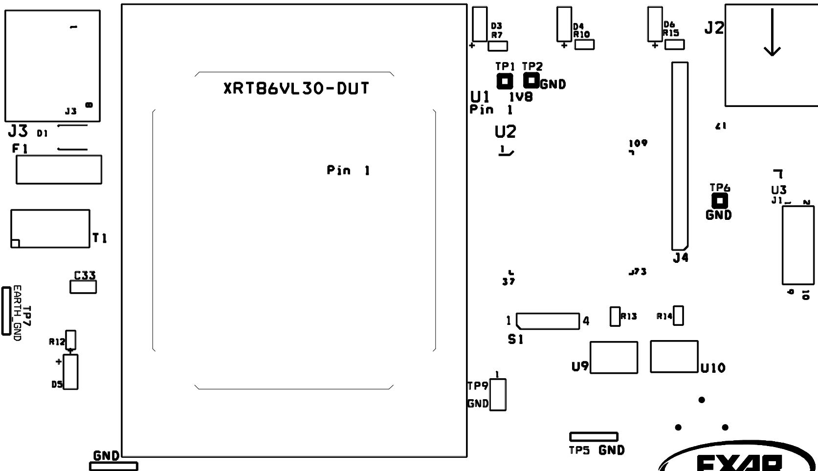
XRT86VL30 (80-pin) EVALUATION BOARD April 2008 Rev 2
