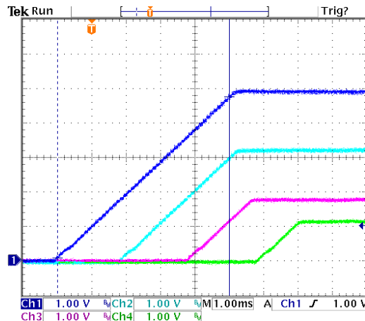
Figure 7 Sequential Start-up
