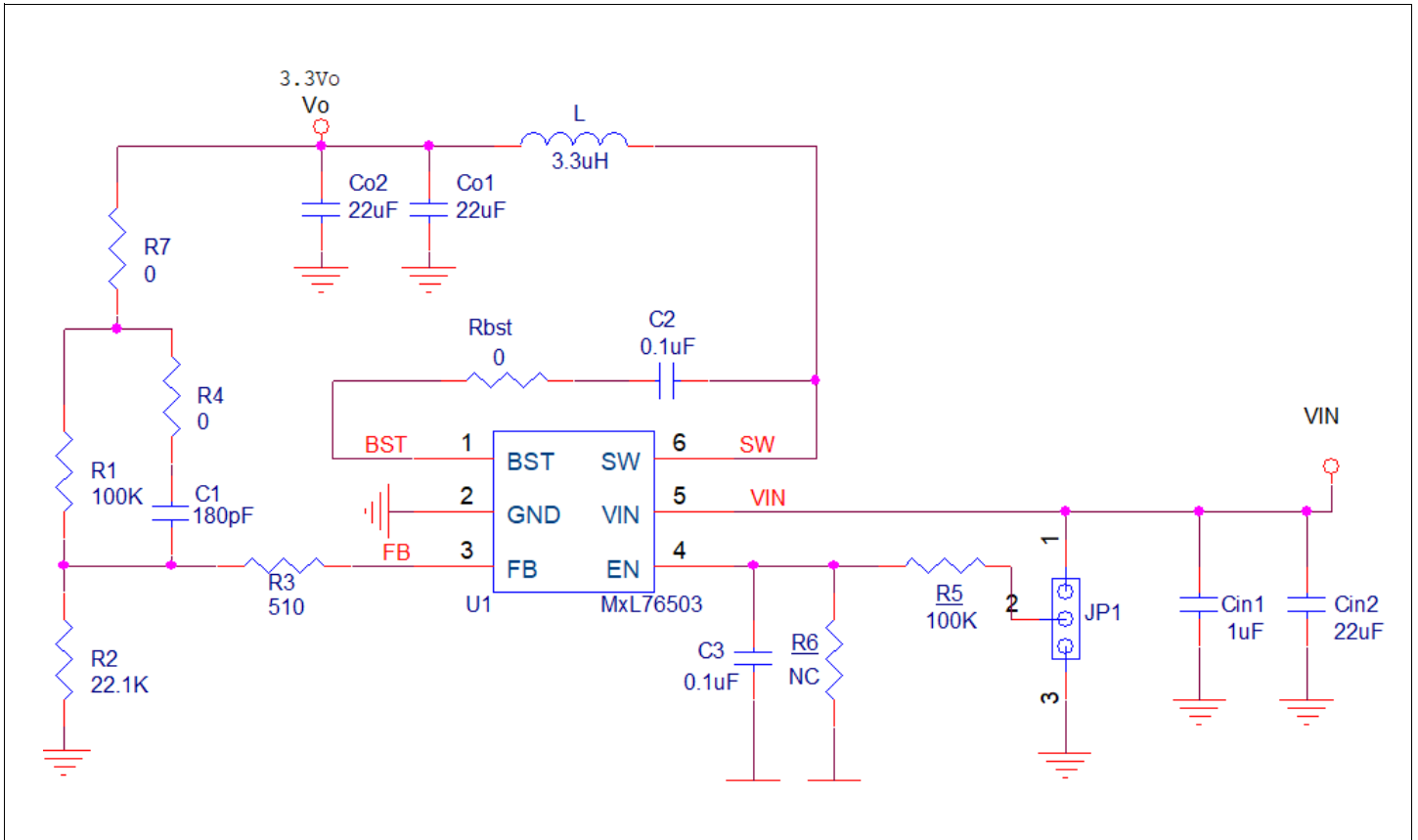
Figure 6: EVK Schematic
