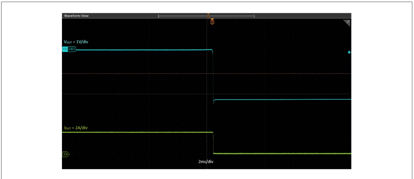
Figure 5: MxL76503 Shutdown with a 3A Load
