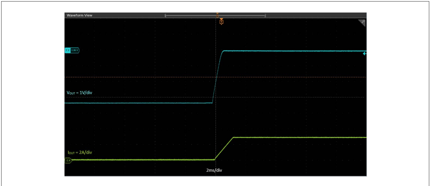
Figure 4: MxL76503 Start-Up with a 3A Load
