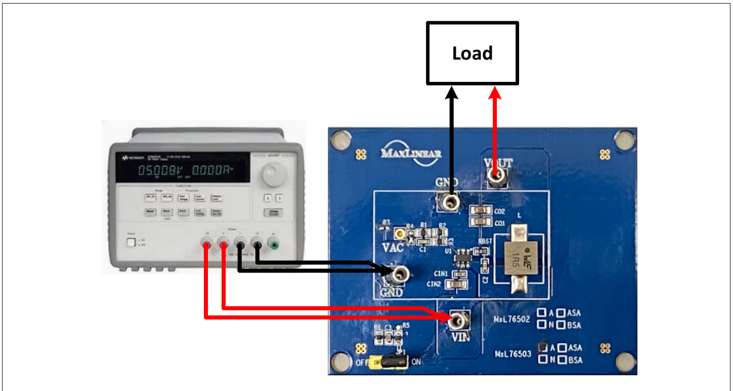
Figure 3: V_{IN} and V_{OUT} Connections of the MxL76503 EVK
