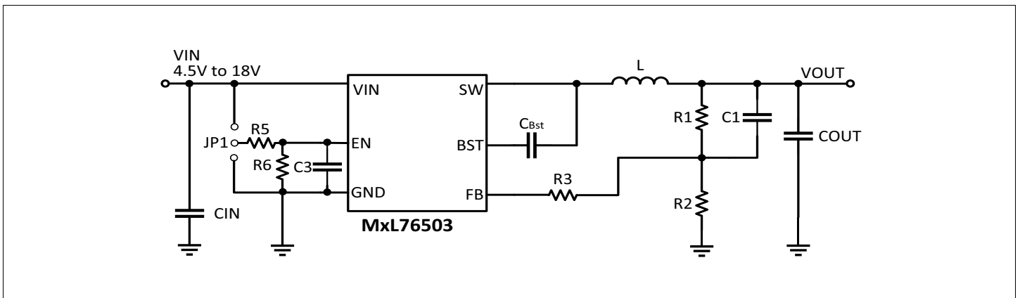
Figure 2: MxL76503 EVK Simplified Block Diagram
