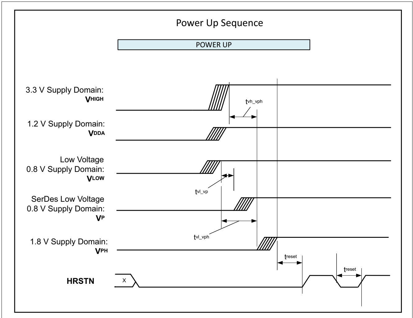
Figure 25 Timing Diagram for the Reset Sequence
