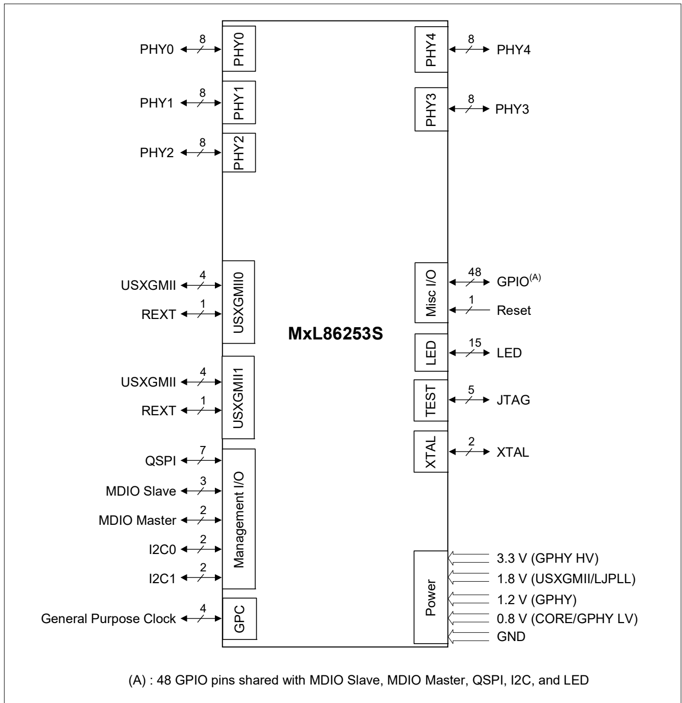
Figure 2 MxL86253S External Signal Overview
