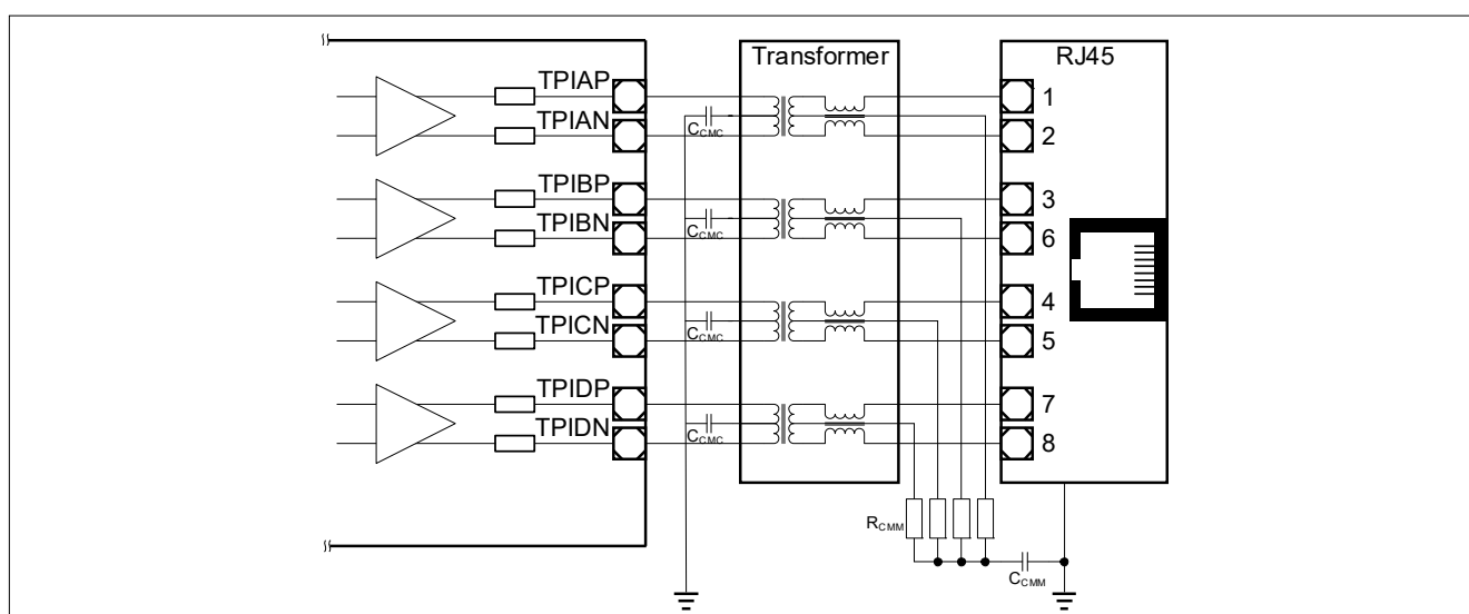
Figure 6 Twisted-Pair Interface of MxL86253S Including Transformer and RJ45 Plug
