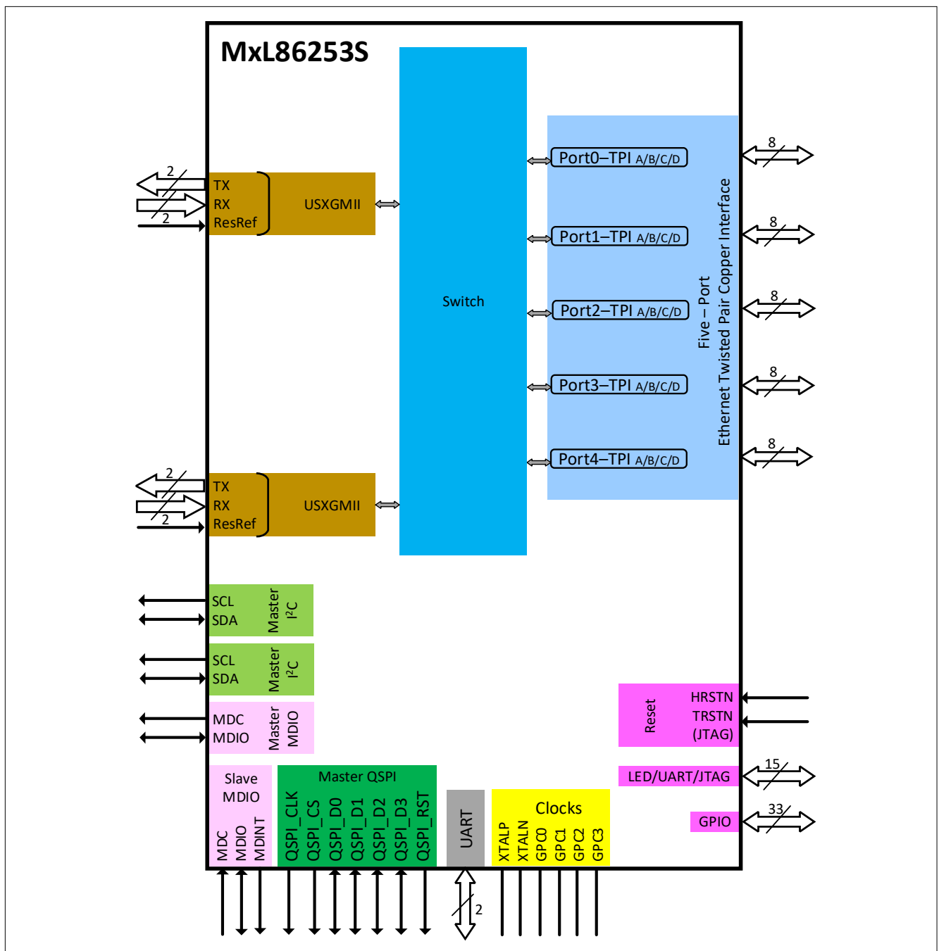
Figure 1 MxL86253S Block Diagram
