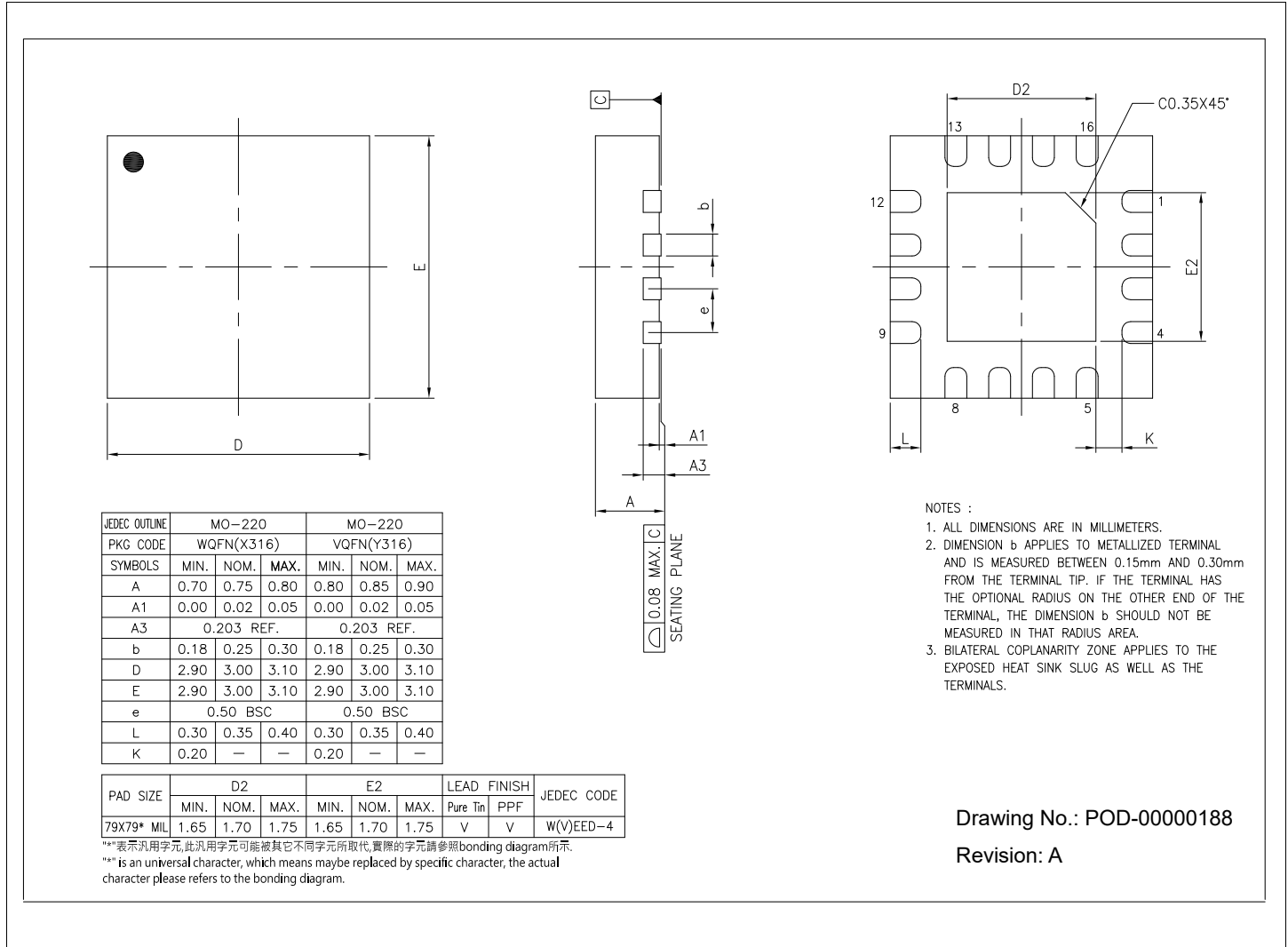
Figure 7: QFN-16 Mechanical Dimensions
