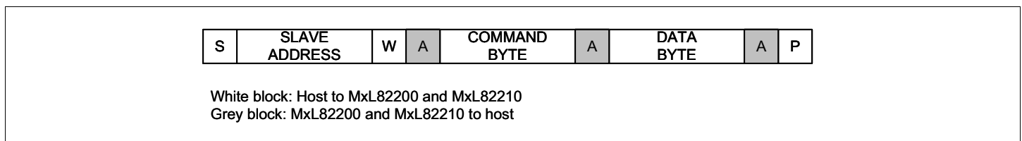
Figure 5: Master Writes To Slave
