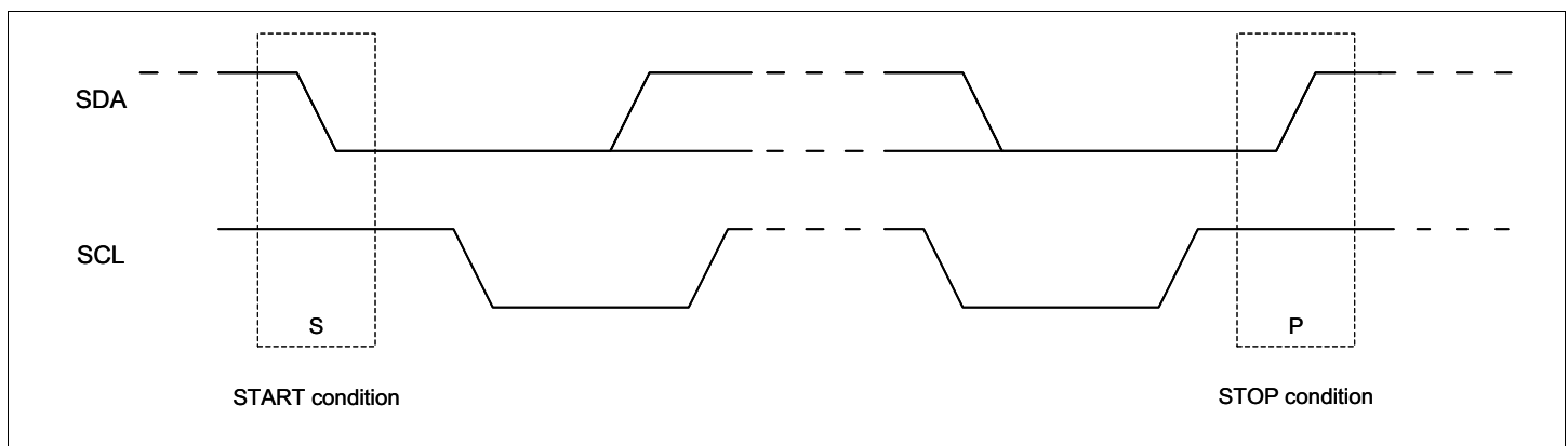
Figure 4: I 2 C Start and Stop Conditions
