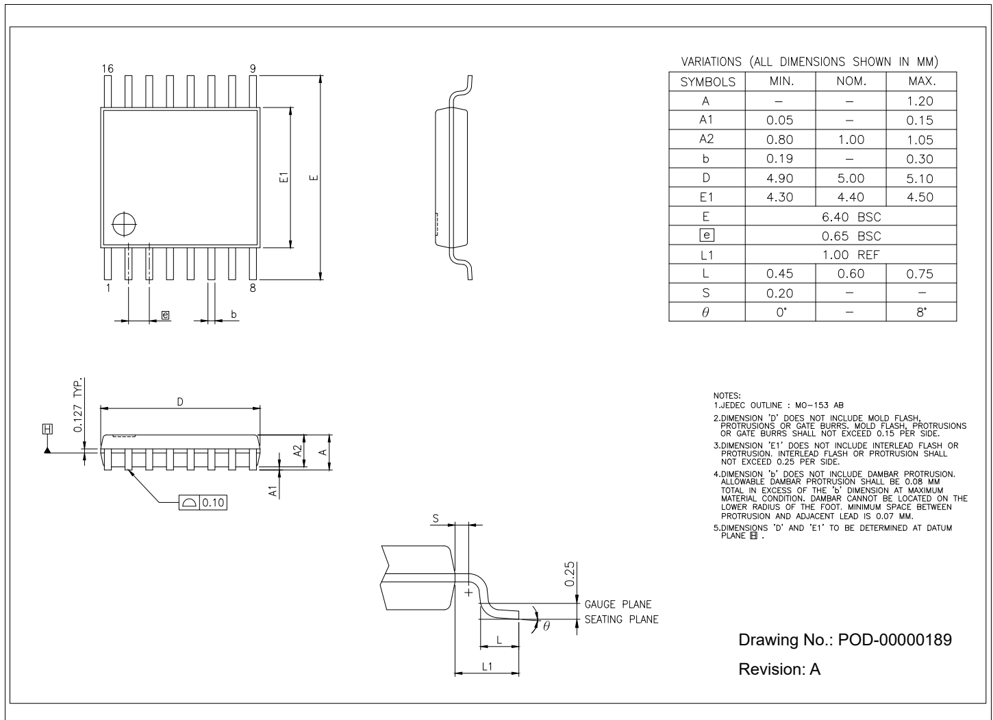
Figure 8: TSSOP-16 Mechanical Dimensions
