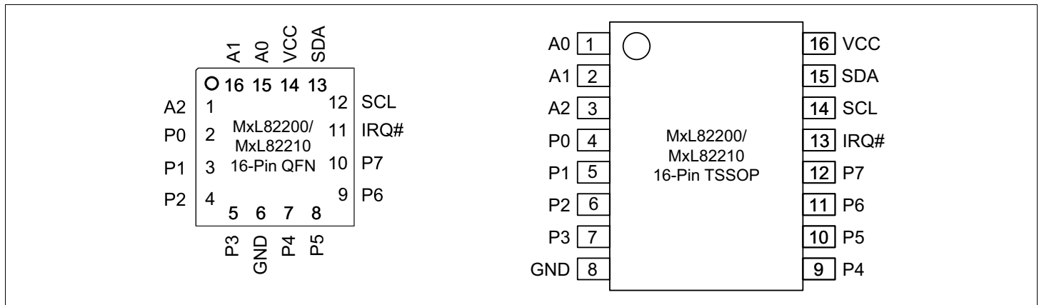
Figure 2: Pin Configuration (Top View)
