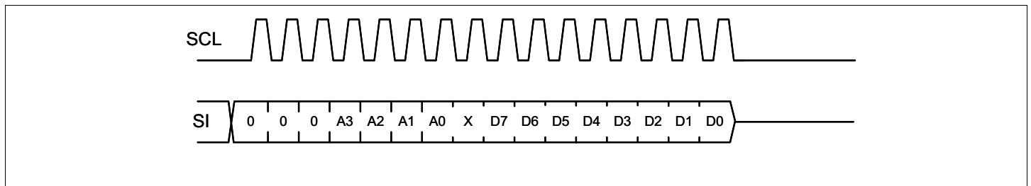
Figure 6: SPI Write
