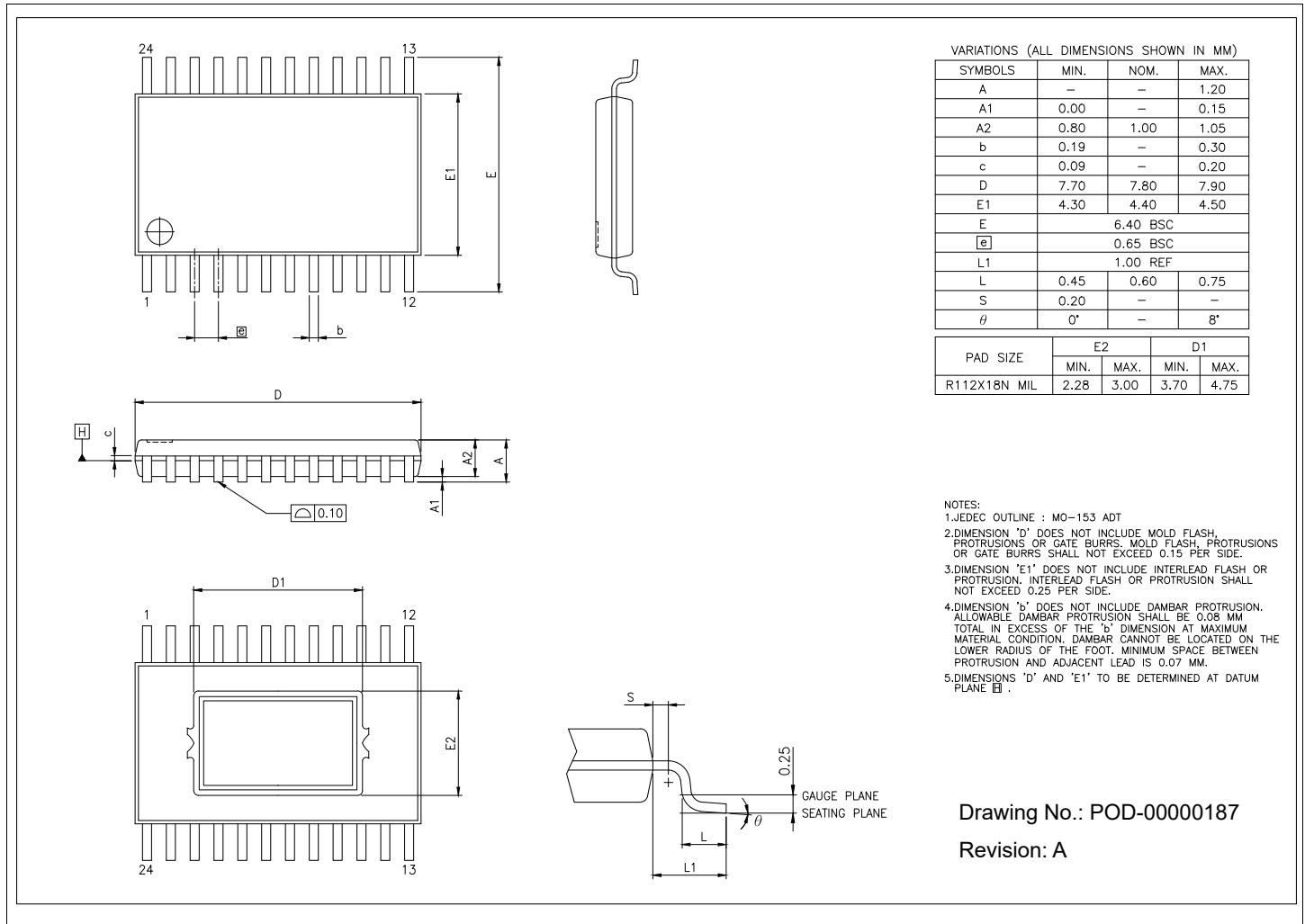
Figure 8: TSSOP-24 Mechanical Dimensions
