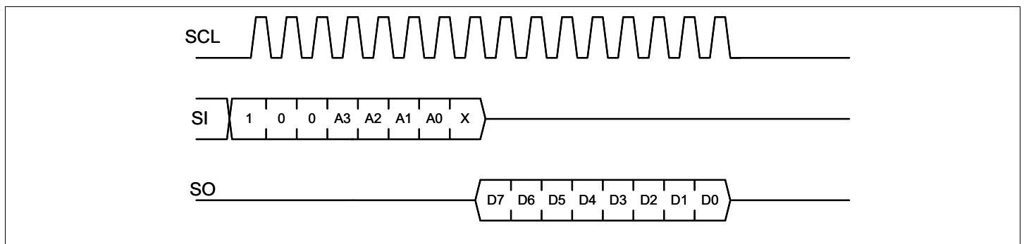
Figure 7: SPI Read
