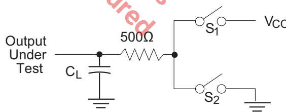
Figure 4. Driver Timing Test Load #2 Circuit
