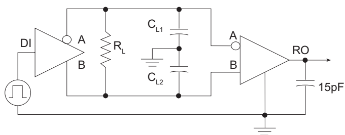
Figure 3. Driver / Receiver Timing Test Circuit
