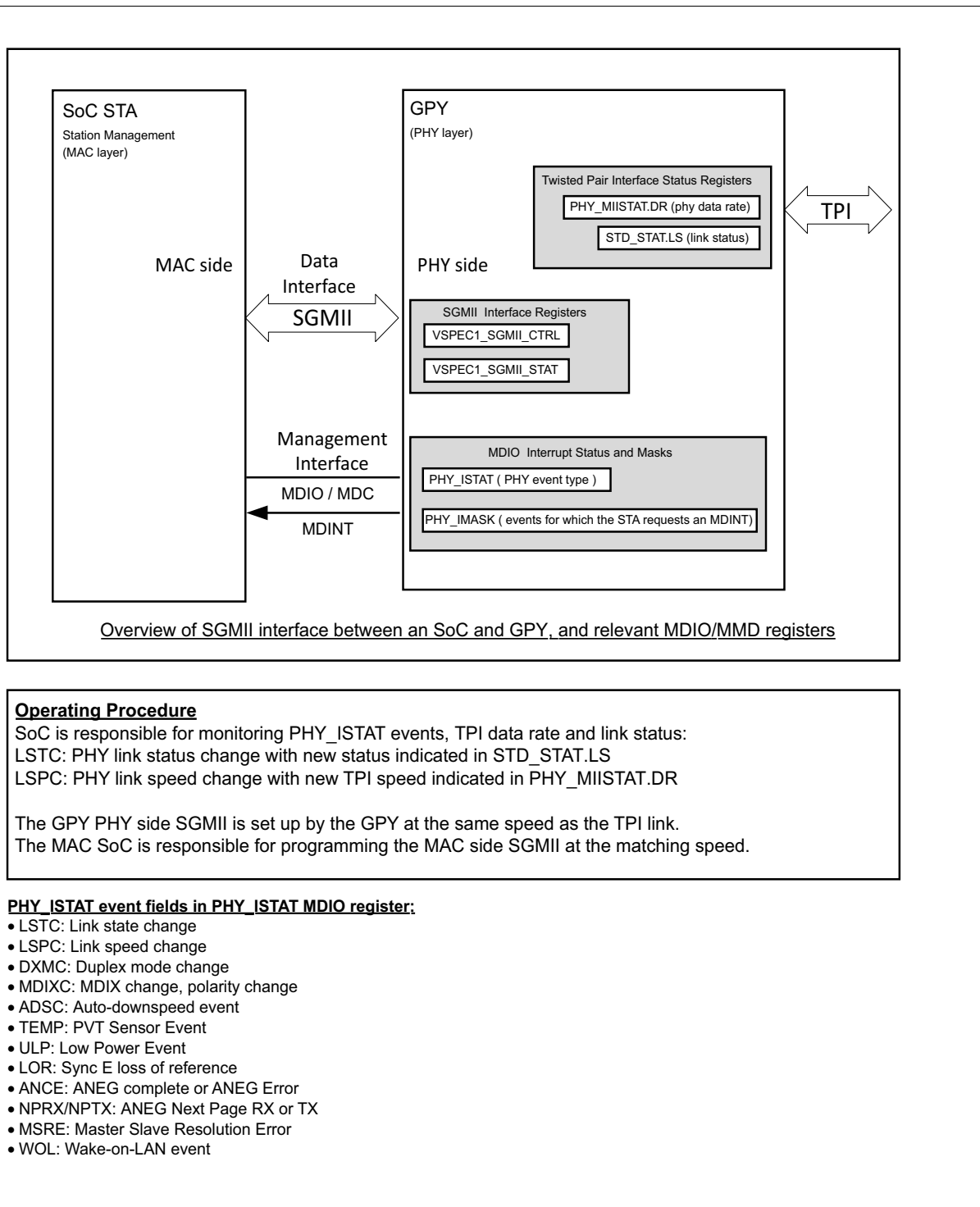
Figure 9 GPY115 SGMII Configuration and Status Registers
