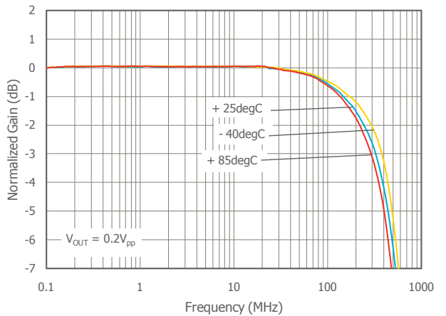
Frequency Response vs. Temperature at V_S = 5\text{V}
