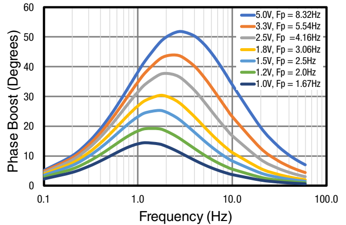
Figure 28: C_{FF} Phase Boost vs. Frequency F_z Zero Normalized to 1
