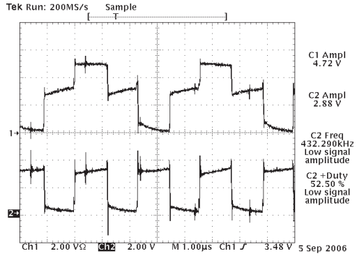
SP3225E/SP3227E Charge Pump Waveforms, Vcc=3.3V, All Channel Switching
