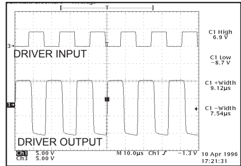
Figure 9. Typical RS-232 Driver Output Waveform
