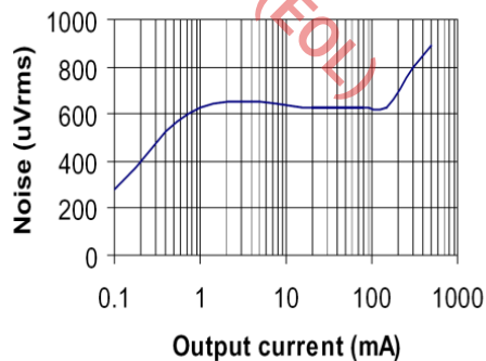
Fig. 20: Output Noise, C_{BYP} = open
