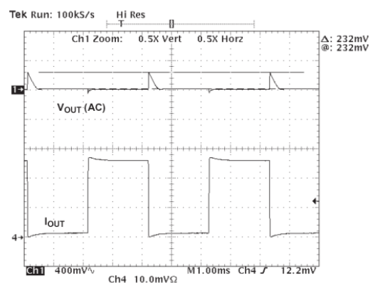
Fig. 8: Load Regulation, I_O=100\mu A \sim 500mA
