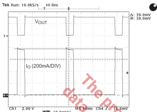
Fig. 4: Current Limit
