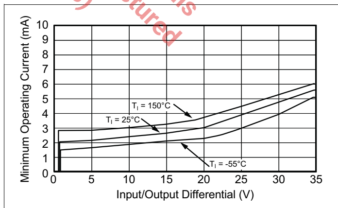
Figure 15: Minimum Operating Current
