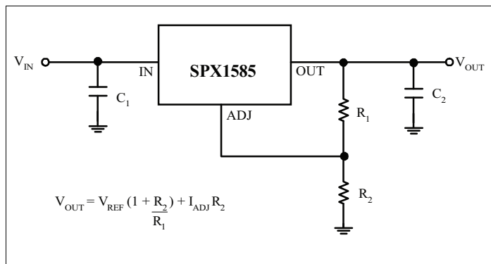
Figure 7: Typical Adjustable Regulator
