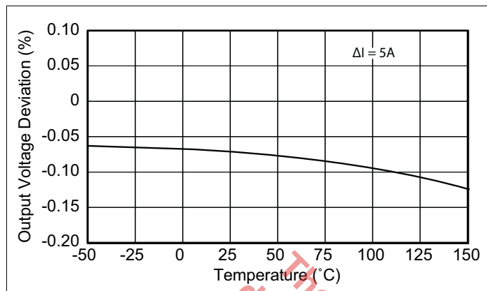
Figure 10: Load Regulation
