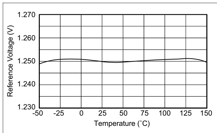
Figure 14: Temperature Stability
