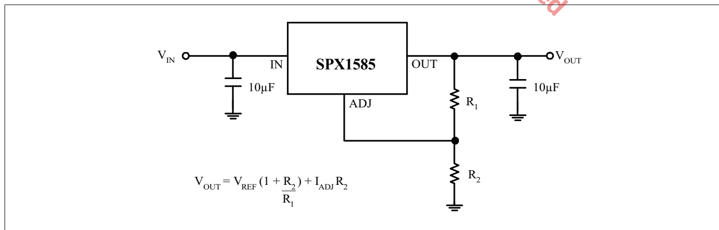
Figure 1: Typical Adjustable Regulator
