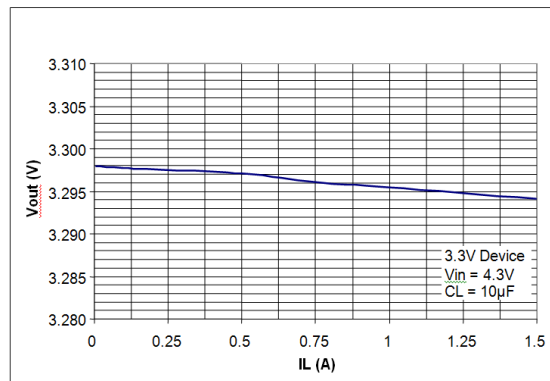
Fig. 5: Load Regulation
