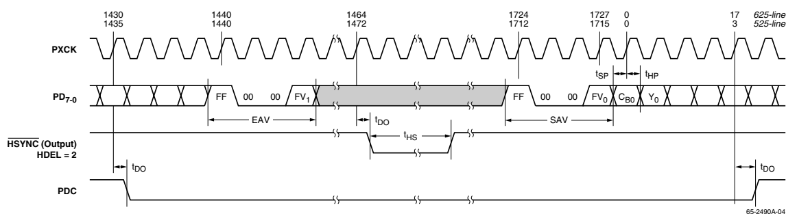
Figure 2b. CCIR-656 Horizontal Interval Timing Detail
