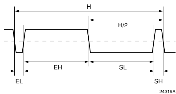
Figure 5. Vertical Sync and Equalization Pulse Detail
