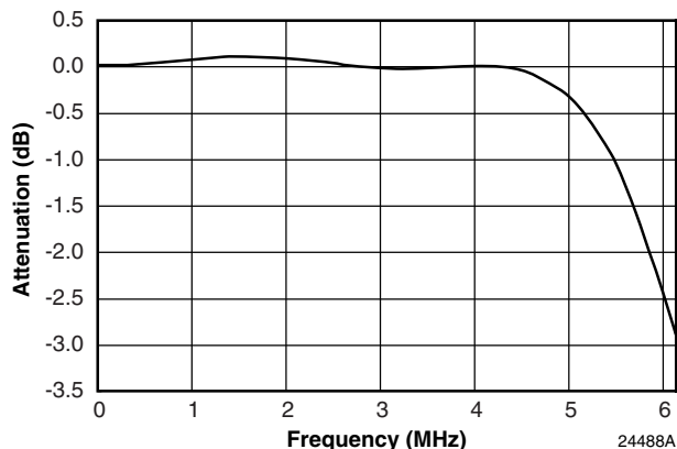
Figure 11. Chrominance and Luminance Interpolation Filter – Passband Detail
