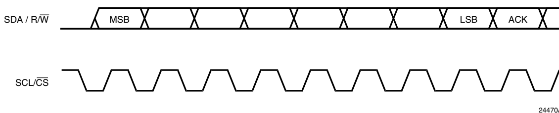
Figure 16. Serial Interface – Typical Byte Transfer
