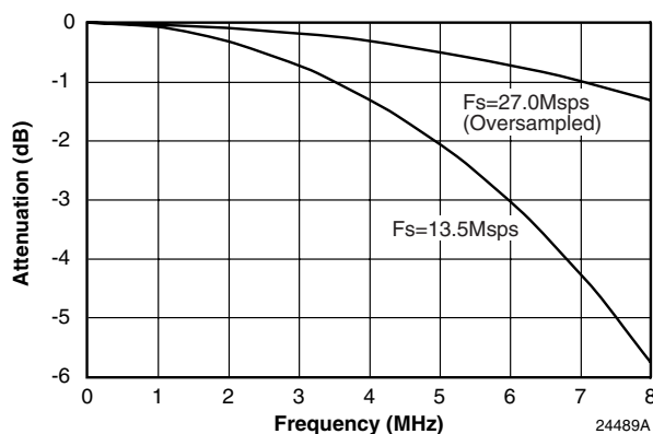
Figure 12. \sin(x)/x Response
