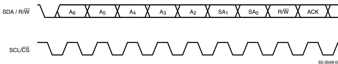
Figure 16A. Chip Address with Read/Write Bit
