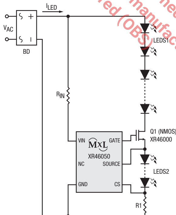
Figure 1. Typical Application
