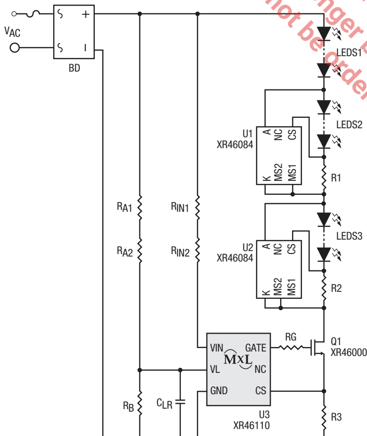
Figure 1. Typical Application
