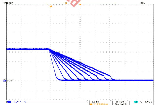
Figure 10: Simultaneous Shut-Down
