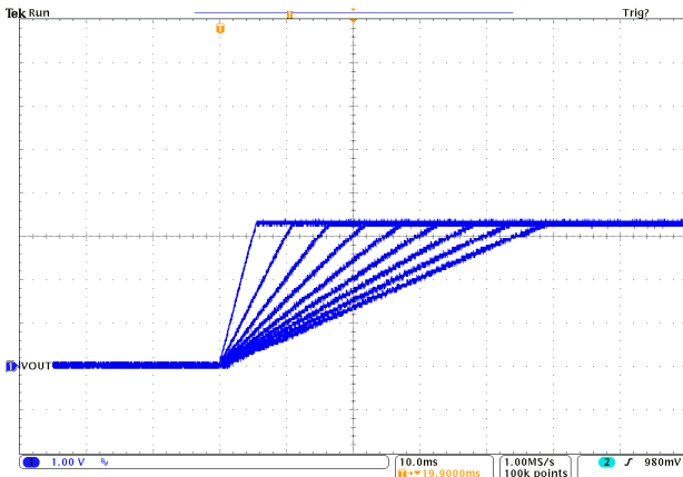
Figure 9: Simultaneous Start-Up
