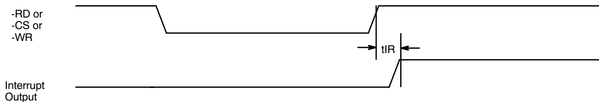
Figure 63. Interrupt Timing
