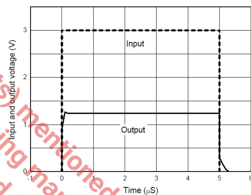
Fig. 12: Pulse Response
