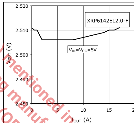
Fig. 7: Load regulation
