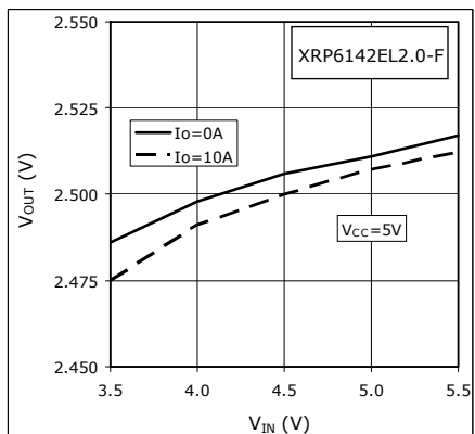
Fig. 8: Line regulation
