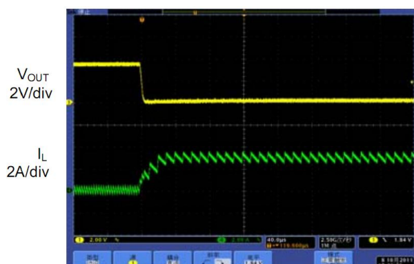
Fig. 14: Short-circuit protection, I_{OUT}=2A Base Time 40 \mu s /div
