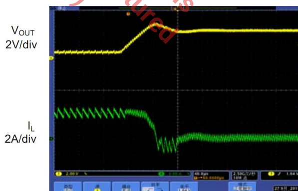
Fig. 15: Short-circuit recovery, I_{OUT}=2A Base Time 40 \mu s /div
