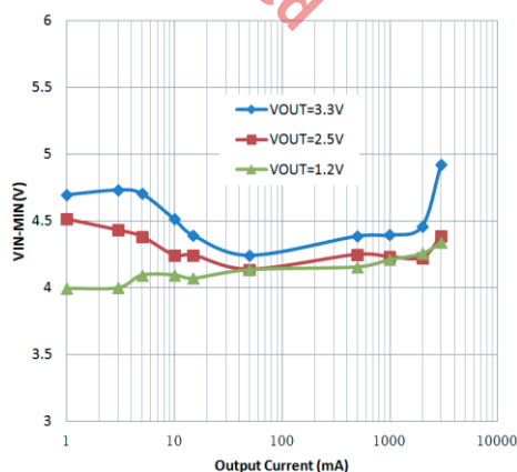
Fig. 9: Minimum Start-Up Voltage vs Output Current
