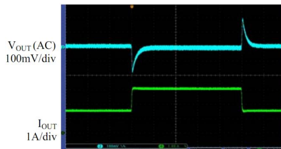
Time 200μs/div Fig. 11: Load transient I_{OUT}=1.5A to 3A
