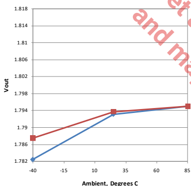
Fig. 18: Temperature Regulation 1.8V out ( \pm 1\% Vout window)
