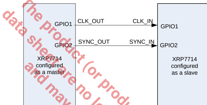
Fig. 28: Master/Slave Configuration of the XRP7714
