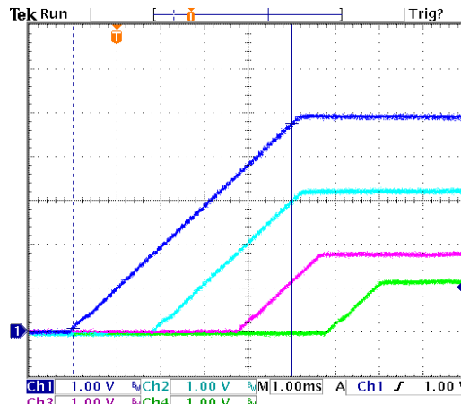
Figure 7 Sequential Start-up
