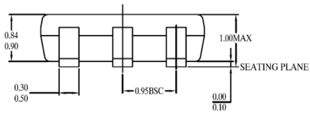
SIDE VIEW - 2
