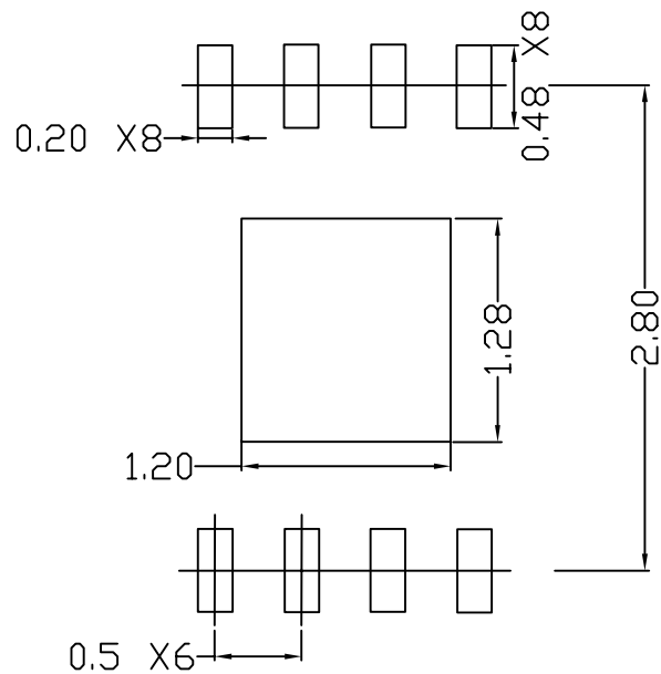
TYPICAL RECOMMENDED STENCIL
