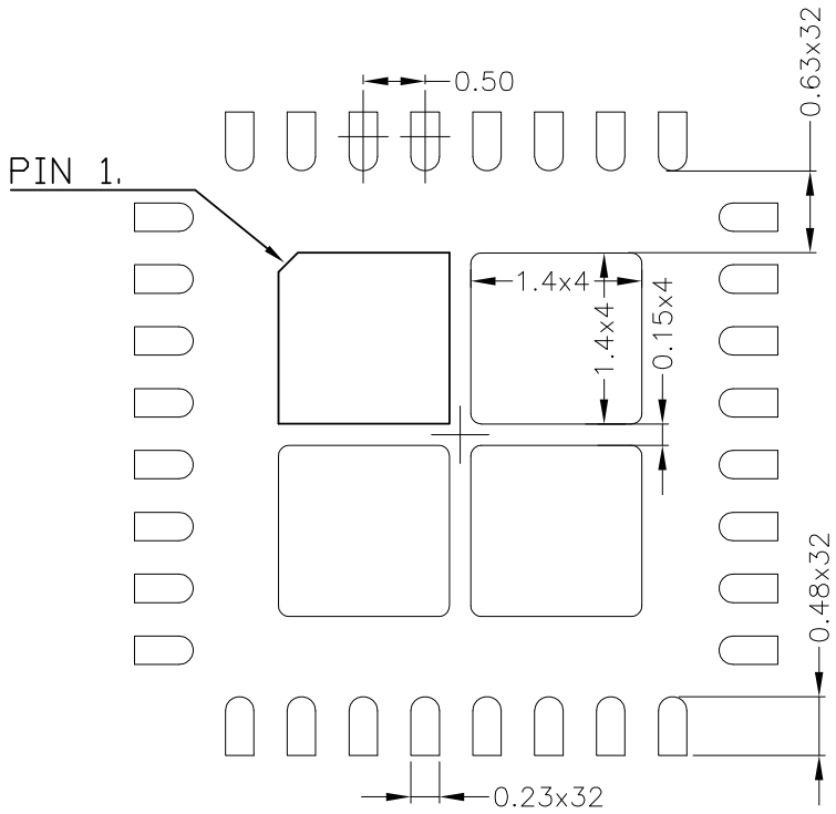
TYPICAL RECOMMENDED STENCIL
