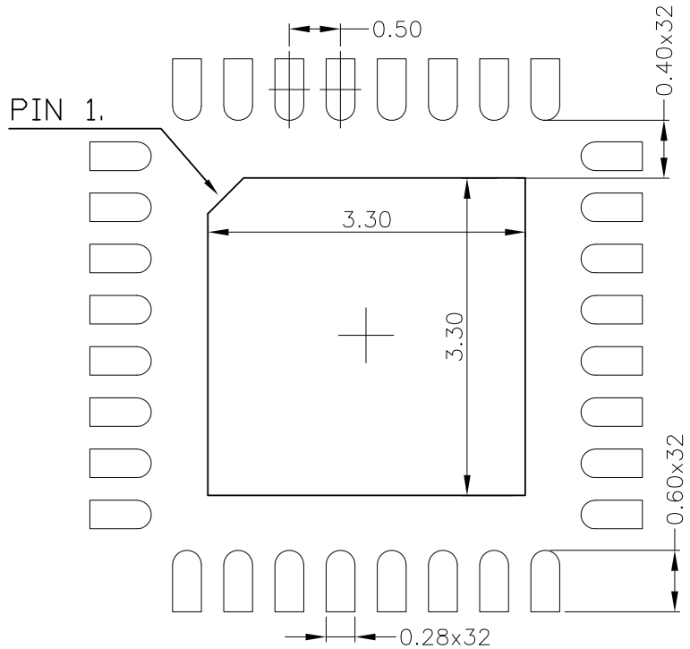
TYPICAL RECOMMENDED LAND PATTERN
