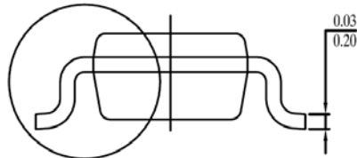
SIDE VIEW-1
