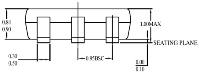
SIDE VIEW - 2
