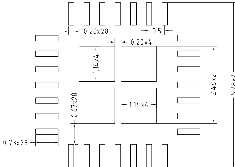
TYPICAL RECOMMENDED STENCIL
