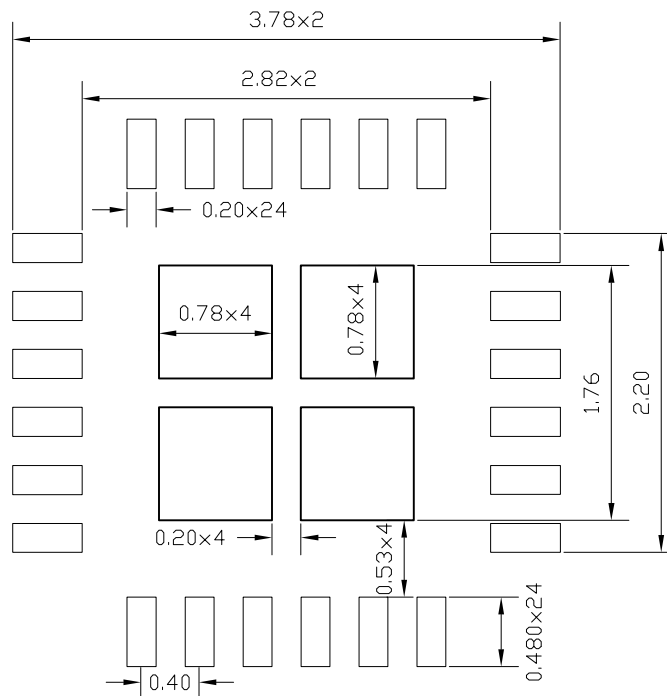
TYPICAL RECOMMENDED STENCIL
